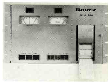
Fig. 4. Auto alarm gives chart record.
