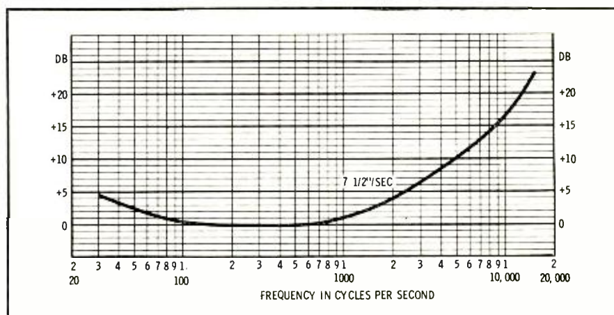
Fig. 3. Typical recording amplifier exhibits frequency response shown by curve.
