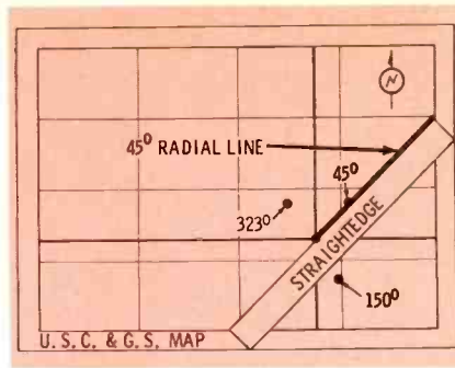
Fig. 3. Drawing radials on survey map.
