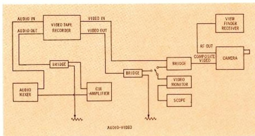
Fig. 1. Unit uses transistorized gear throughout to obtain low power consumption.
