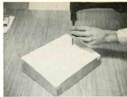
Fig. 3. Layout is used as a template.
